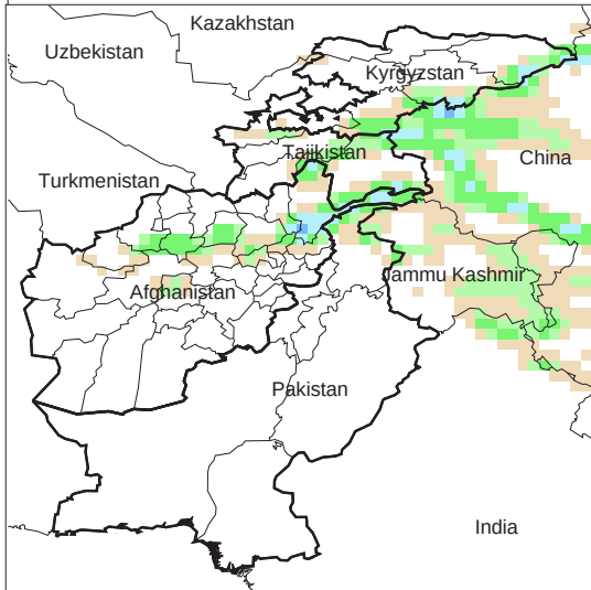
Daily Precip. Forecast for 7 Mar., 2010
