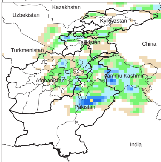
Daily Precip. Forecast for 9 Mar., 2010
