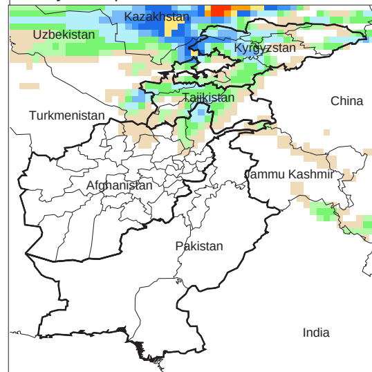
Daily Precip. Forecast for 10 Mar., 2010
