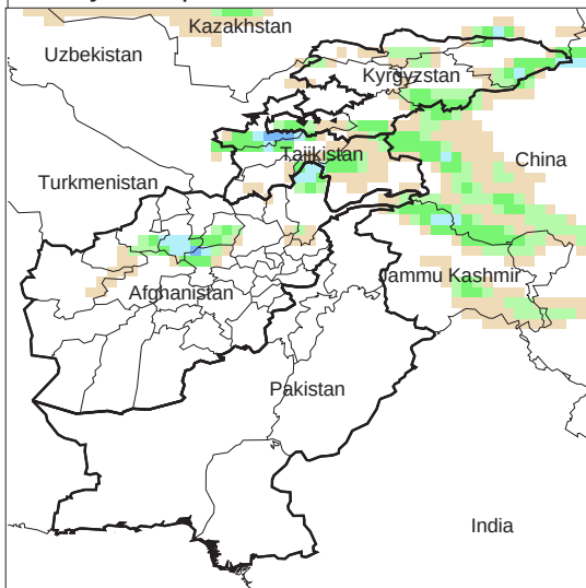
Daily Precip. Forecast for 8 Mar., 2010
