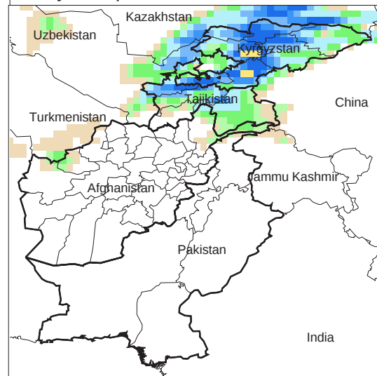
Daily Precip. Forecast for 23 Mar., 2010
