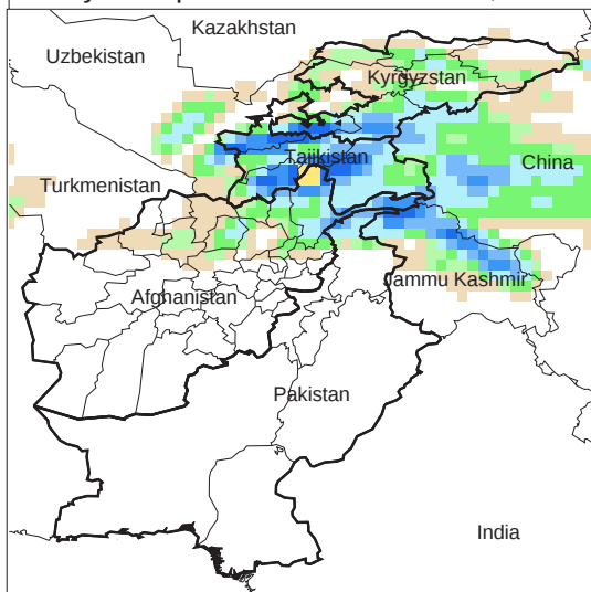
Daily Precip. Forecast for 22 Mar., 2010
