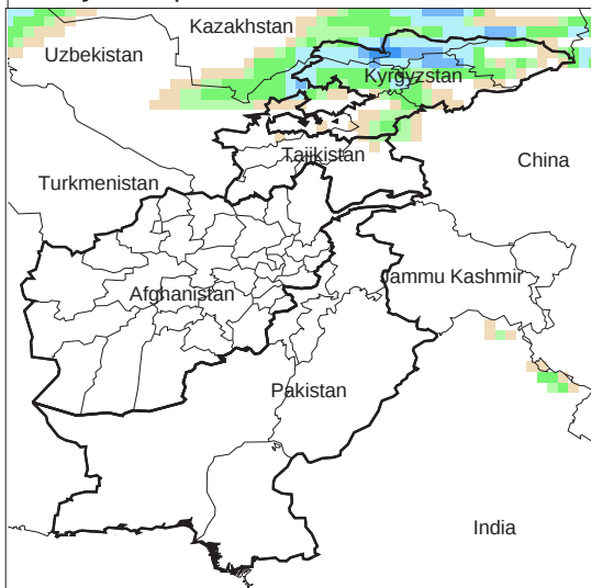
Daily Precip. Forecast for 21 Mar., 2010
