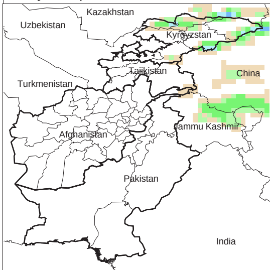
Daily Precip. Forecast for 24 Mar., 2010
