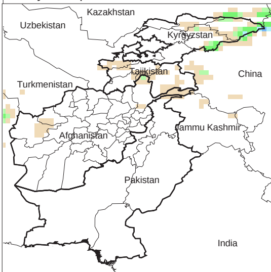
Daily Precip. Forecast for 25 Mar., 2010
