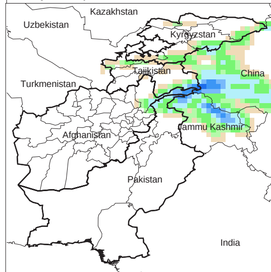
Daily Precip. Forecast for 26 Mar., 2010
