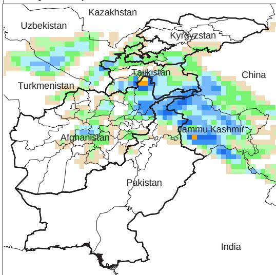
Daily Precip. Forecast for 1 Apr., 2010
