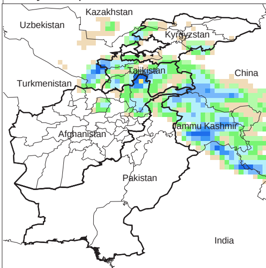
Daily Precip. Forecast for 2 Apr., 2010
