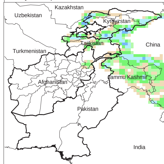
Daily Precip. Forecast for 3 Apr., 2010
