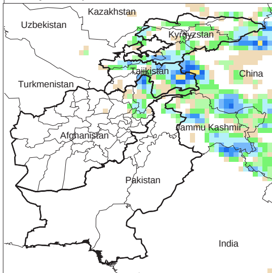
Daily Precip. Forecast for 16 Jun., 2010
