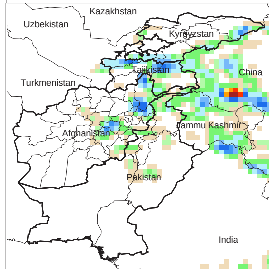
Daily Precip. Forecast for 17 Jun., 2010
