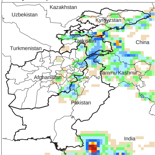
Daily Precip. Forecast for 15 Jun., 2010
