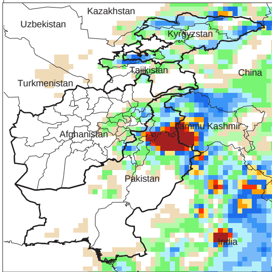
Daily Precip. Forecast for 24 Jul., 2010
