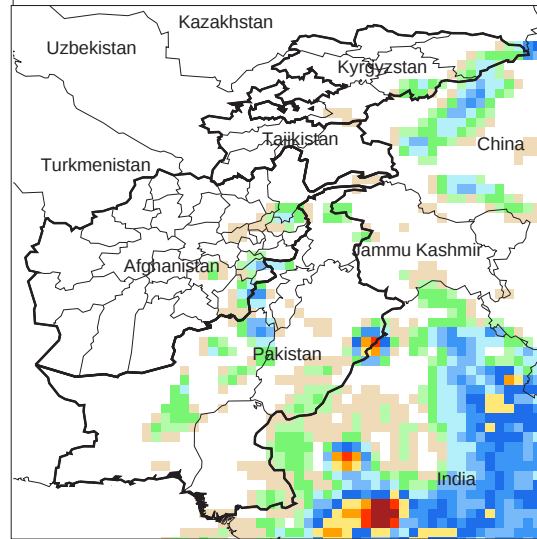
Daily Precip. Forecast for 26 Jul., 2010
