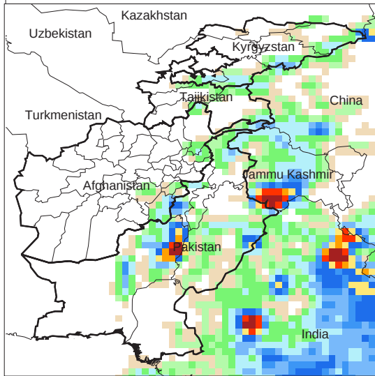
Daily Precip. Forecast for 25 Jul., 2010
