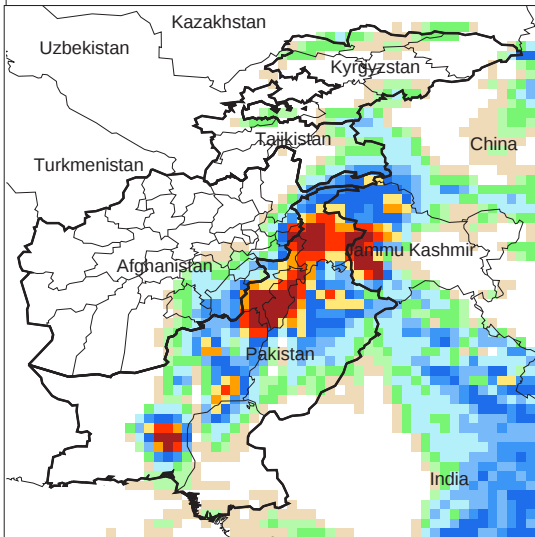
Daily Precip. Forecast for 1 Aug., 2010
