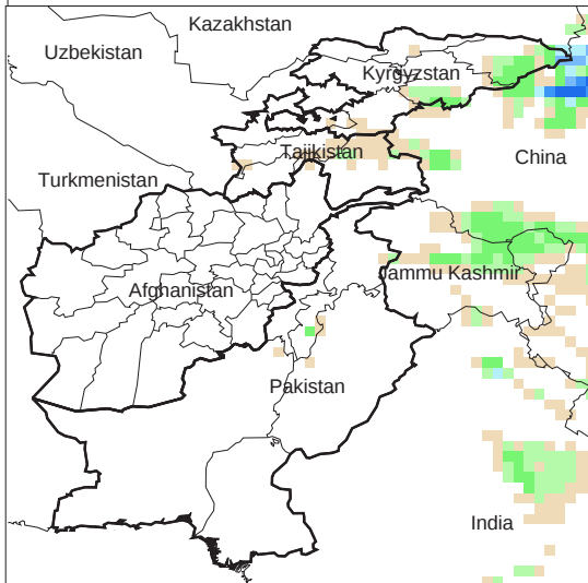
Daily Precip. Forecast for 26 Oct., 2010
