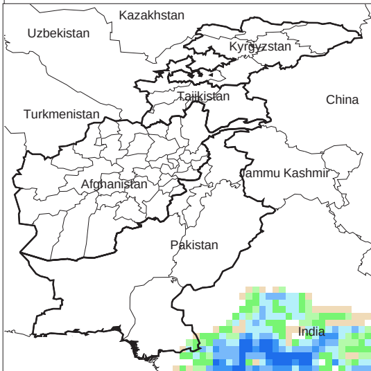
Daily Precip. Forecast for 11 Nov., 2010
