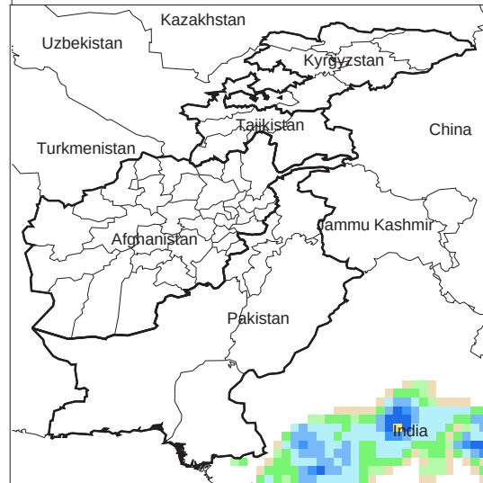
Daily Precip. Forecast for 12 Nov., 2010
