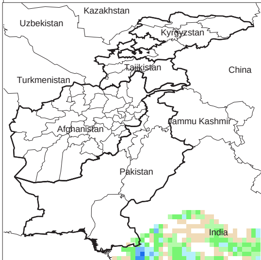
Daily Precip. Forecast for 10 Nov., 2010
