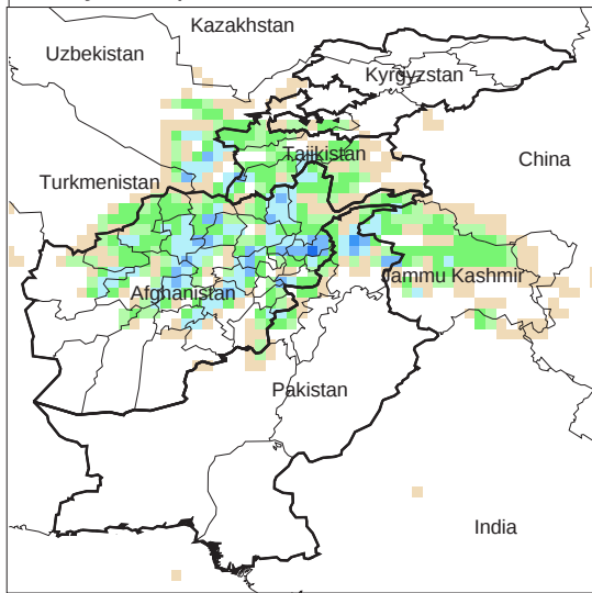
Daily Precip. Forecast for 16 Jan., 2011
