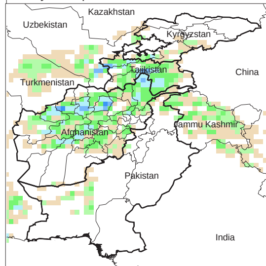
Daily Precip. Forecast for 17 Jan., 2011
