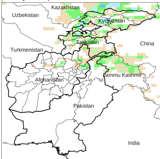
Daily Precip. Forecast for 22 Jan., 2011
