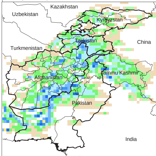
Daily Precip. Forecast for 3 Mar., 2011
