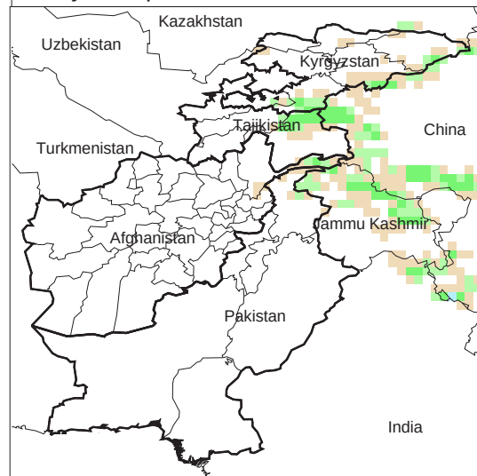
Daily Precip. Forecast for 25 Mar., 2011
