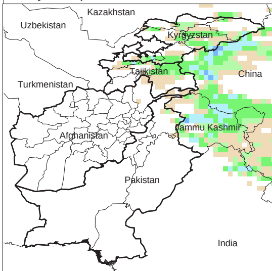
Daily Precip. Forecast for 23 Mar., 2011
