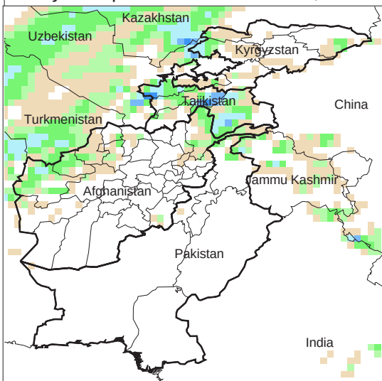
Daily Precip. Forecast for 24 Mar., 2011
