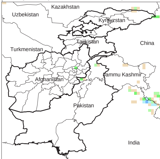
Daily Precip. Forecast for 26 Apr., 2011
