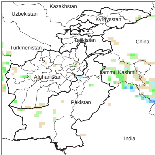
Daily Precip. Forecast for 2 May, 2011
