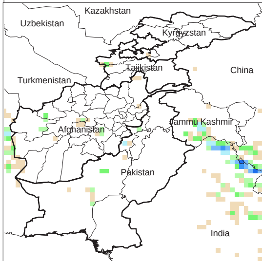
Daily Precip. Forecast for 3 May, 2011
