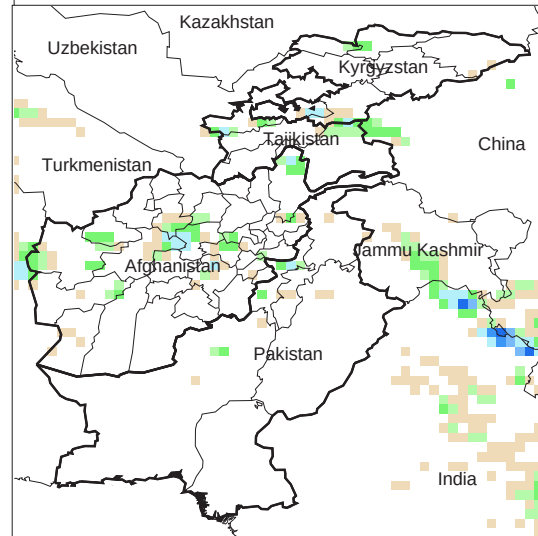
Daily Precip. Forecast for 4 May, 2011
