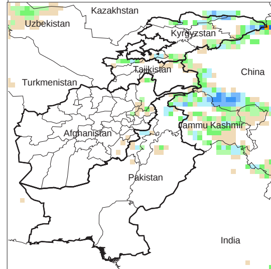
Daily Precip. Forecast for 13 May, 2011
