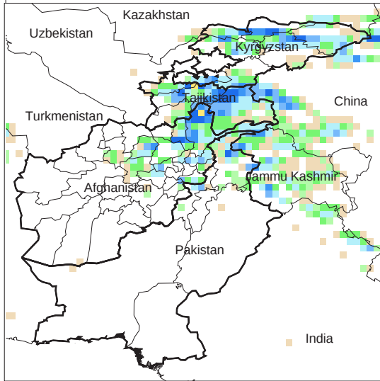
Daily Precip. Forecast for 12 May, 2011
