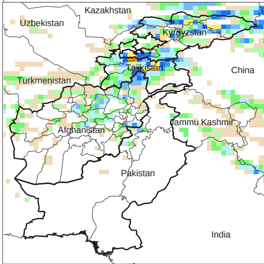
Daily Precip. Forecast for 11 May, 2011
