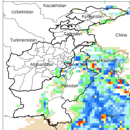
Daily Precip. Forecast for 28 Aug., 2011
