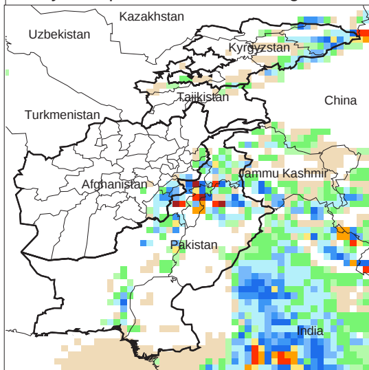
Daily Precip. Forecast for 27 Aug., 2011
