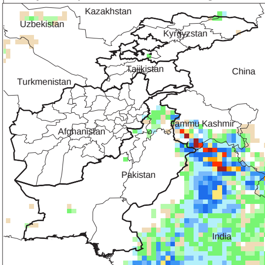
Daily Precip. Forecast for 26 Aug., 2011
