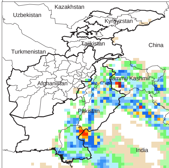
Daily Precip. Forecast for 8 Sep., 2011
