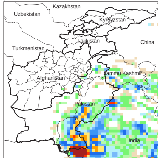
Daily Precip. Forecast for 9 Sep., 2011
