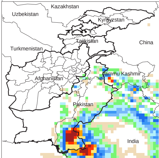
Daily Precip. Forecast for 7 Sep., 2011
