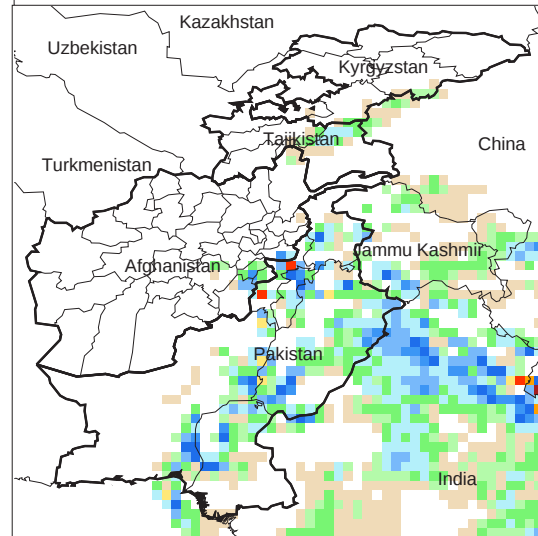
Daily Precip. Forecast for 14 Sep., 2011
