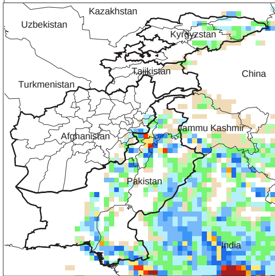
Daily Precip. Forecast for 13 Sep., 2011
