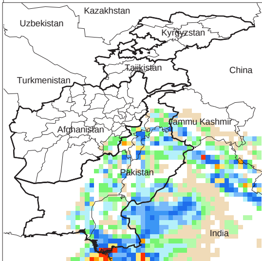
Daily Precip. Forecast for 12 Sep., 2011
