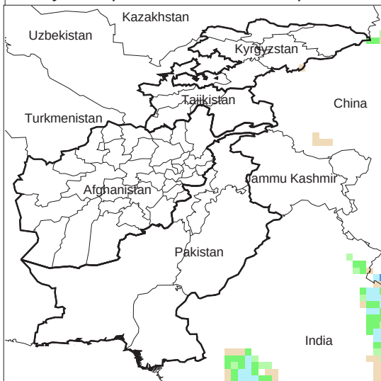
Daily Precip. Forecast for 24 Sep., 2011
