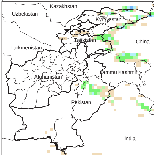
Daily Precip. Forecast for 29 Sep., 2011
