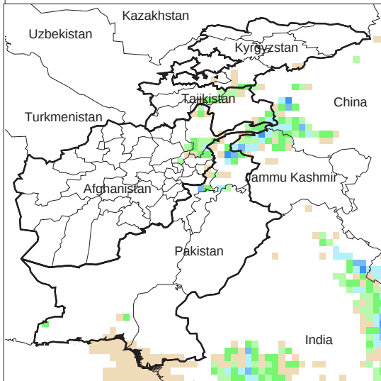
Daily Precip. Forecast for 28 Sep., 2011
