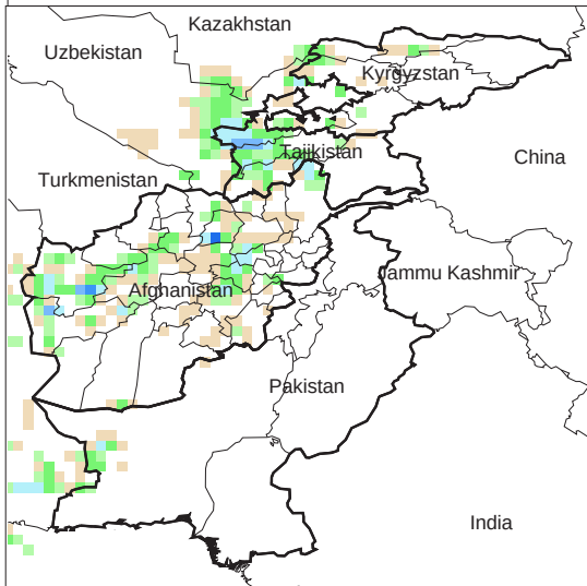
Daily Precip. Forecast for 15 Oct., 2011
