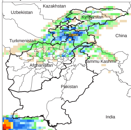
Daily Precip. Forecast for 31 Oct., 2011
