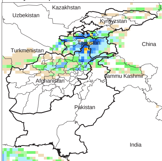
Daily Precip. Forecast for 30 Oct., 2011
