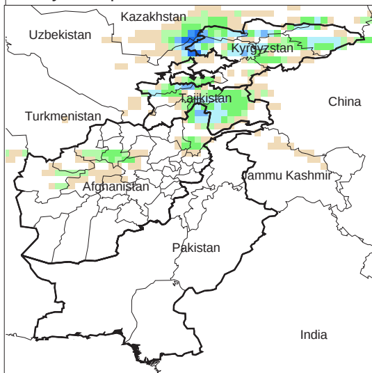
Daily Precip. Forecast for 19 Nov., 2011
