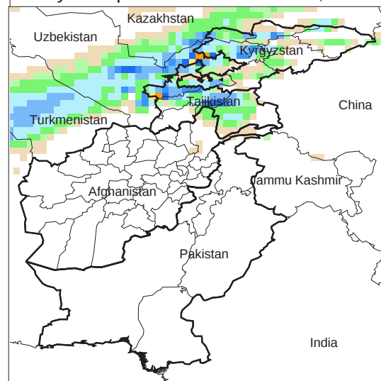
Daily Precip. Forecast for 20 Nov., 2011
