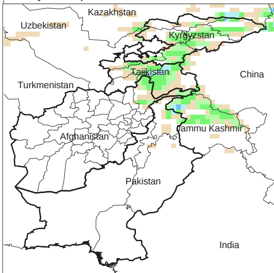
Daily Precip. Forecast for 18 Nov., 2011
