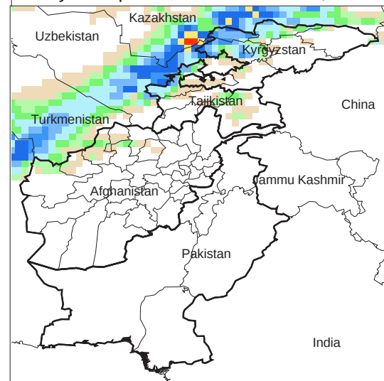
Daily Precip. Forecast for 22 Nov., 2011
