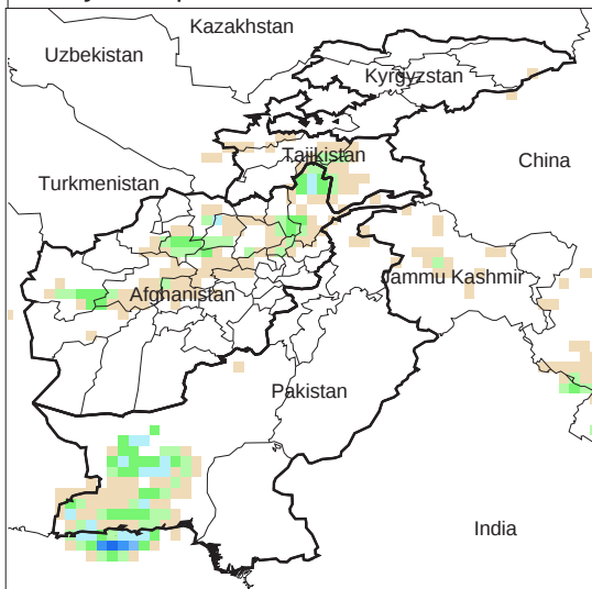
Daily Precip. Forecast for 13 Jan., 2012
