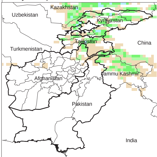
Daily Precip. Forecast for 10 Feb., 2012
