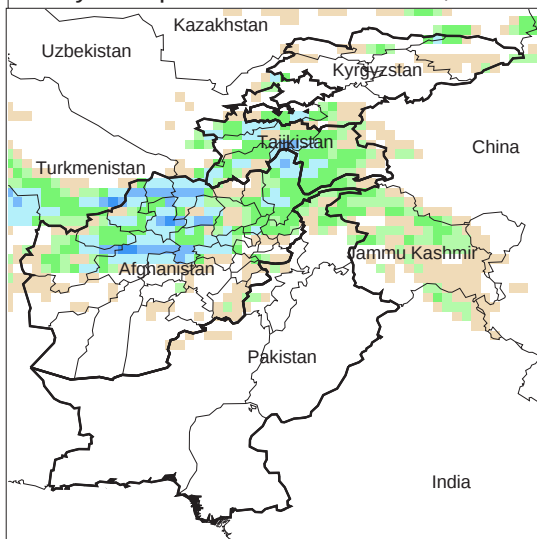
Daily Precip. Forecast for 11 Feb., 2012
