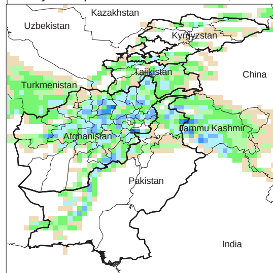
Daily Precip. Forecast for 12 Feb., 2012
