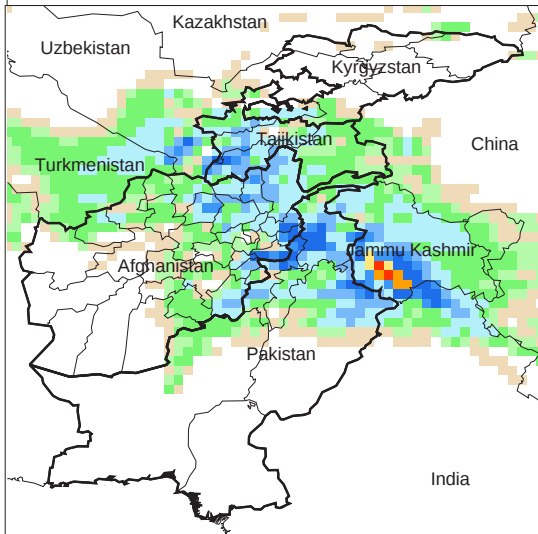
Daily Precip. Forecast for 15 Feb., 2012
