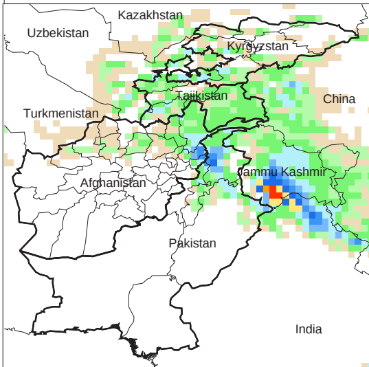
Daily Precip. Forecast for 16 Feb., 2012
