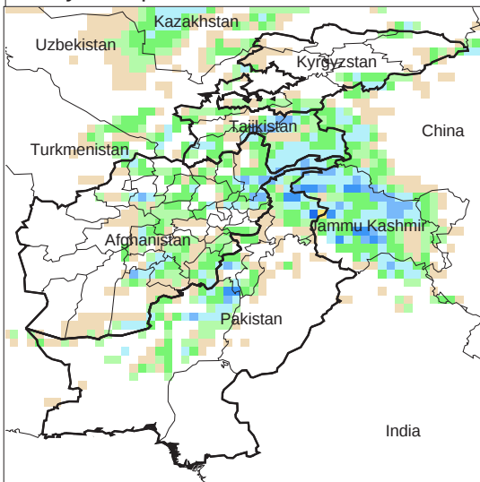
Daily Precip. Forecast for 25 Mar., 2012
