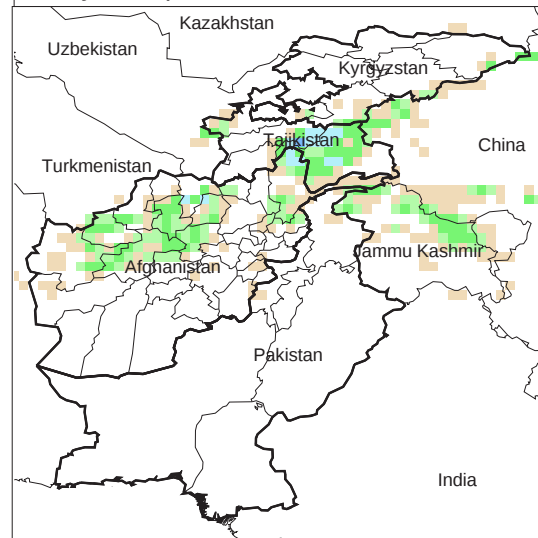
Daily Precip. Forecast for 26 Mar., 2012
