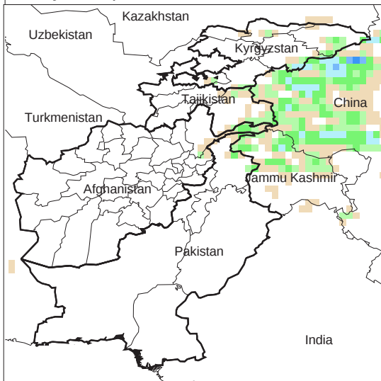
Daily Precip. Forecast for 24 Mar., 2012
