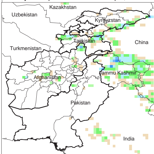
Daily Precip. Forecast for 5 Apr., 2012
