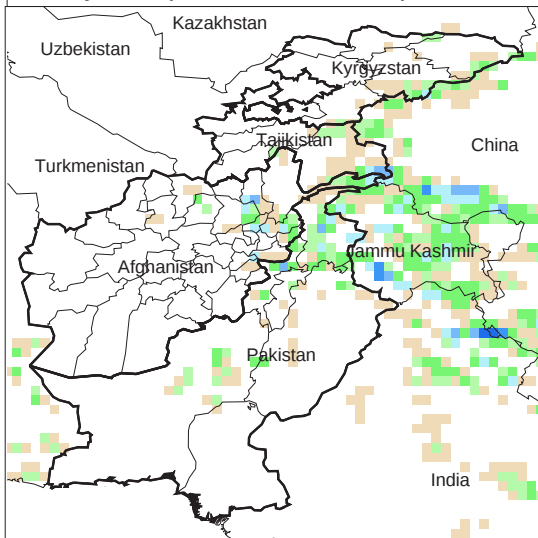
Daily Precip. Forecast for 6 Apr., 2012
