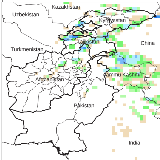
Daily Precip. Forecast for 8 Apr., 2012
