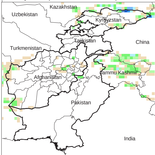
Daily Precip. Forecast for 7 Apr., 2012
