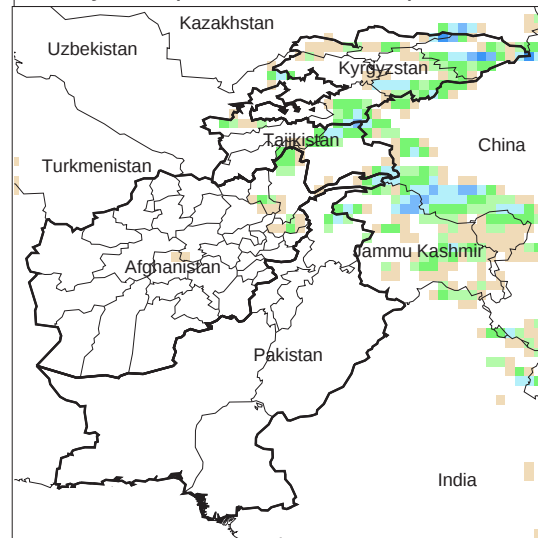
Daily Precip. Forecast for 9 Apr., 2012
