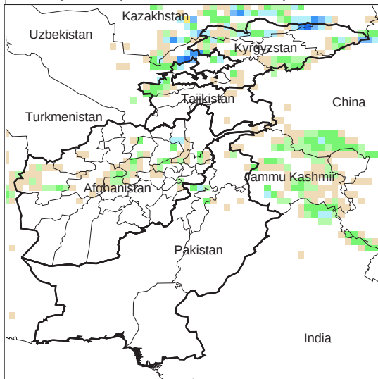
Daily Precip. Forecast for 10 Apr., 2012
