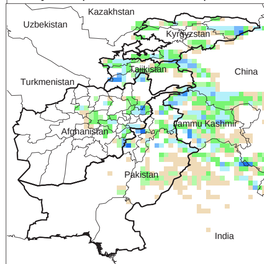
Daily Precip. Forecast for 11 Apr., 2012
