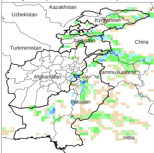
Daily Precip. Forecast for 12 Apr., 2012
