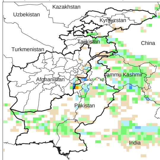
Daily Precip. Forecast for 16 Apr., 2012
