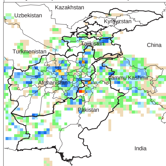
Daily Precip. Forecast for 21 Apr., 2012
