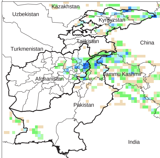
Daily Precip. Forecast for 14 May, 2012
