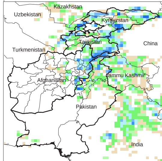
Daily Precip. Forecast for 15 May, 2012
