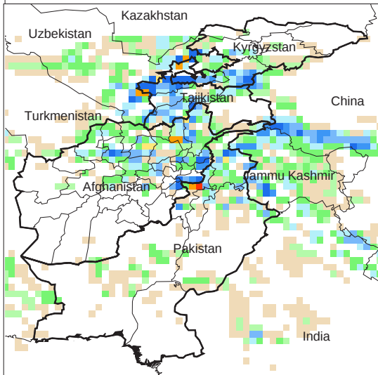
Daily Precip. Forecast for 13 May, 2012
