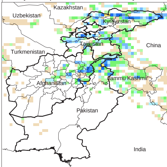
Daily Precip. Forecast for 18 May, 2012
