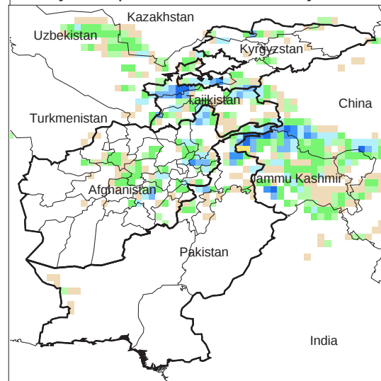
Daily Precip. Forecast for 20 May, 2012
