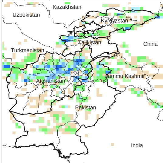
Daily Precip. Forecast for 19 May, 2012
