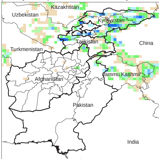
Daily Precip. Forecast for 28 May, 2012
