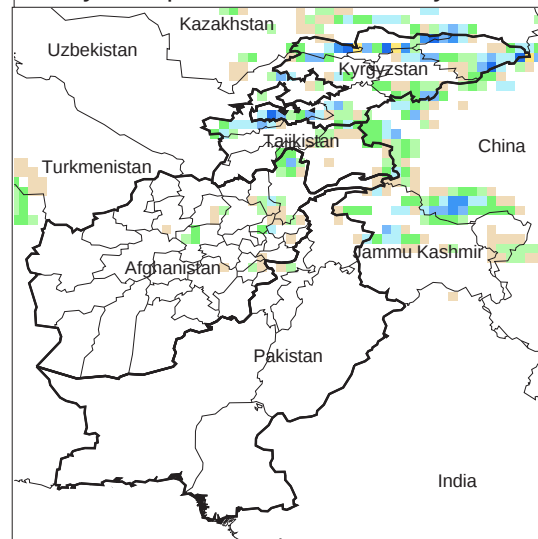
Daily Precip. Forecast for 30 May, 2012
