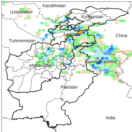
Daily Precip. Forecast for 29 May, 2012
