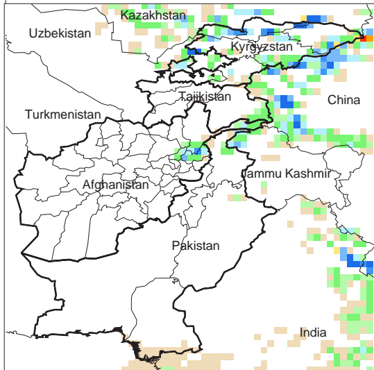
Daily Precip. Forecast for 28 Jun., 2012
