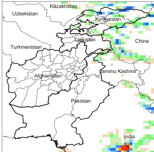
Daily Precip. Forecast for 29 Jun., 2012
