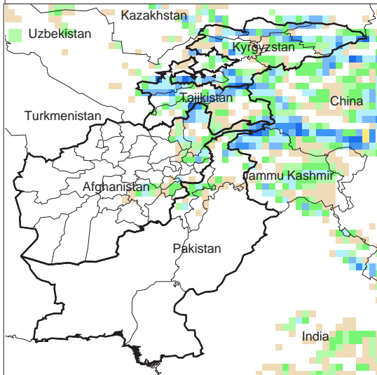
Daily Precip. Forecast for 27 Jun., 2012
