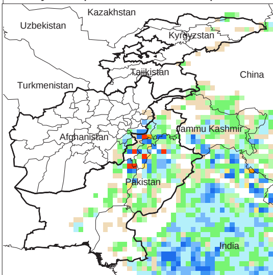
Daily Precip. Forecast for 5 Sep., 2012
