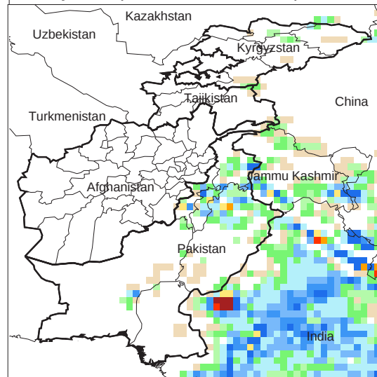
Daily Precip. Forecast for 6 Sep., 2012
