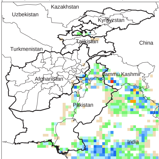
Daily Precip. Forecast for 4 Sep., 2012
