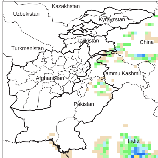
Daily Precip. Forecast for 23 Sep., 2012
