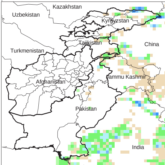
Daily Precip. Forecast for 22 Sep., 2012
