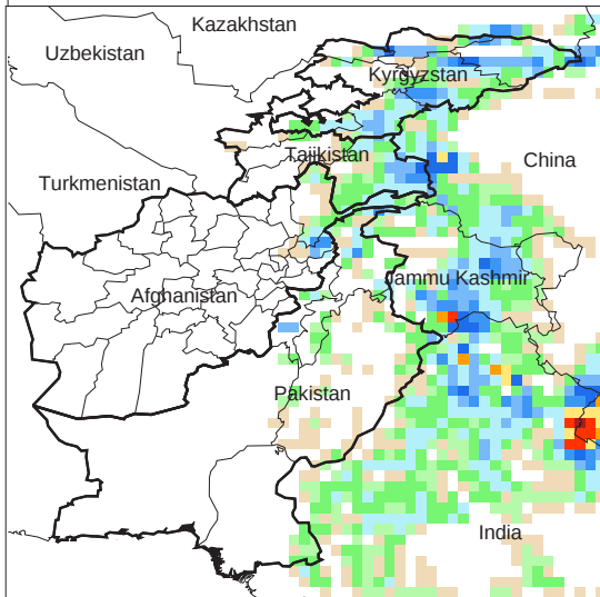
Daily Precip. Forecast for 21 Sep., 2012
