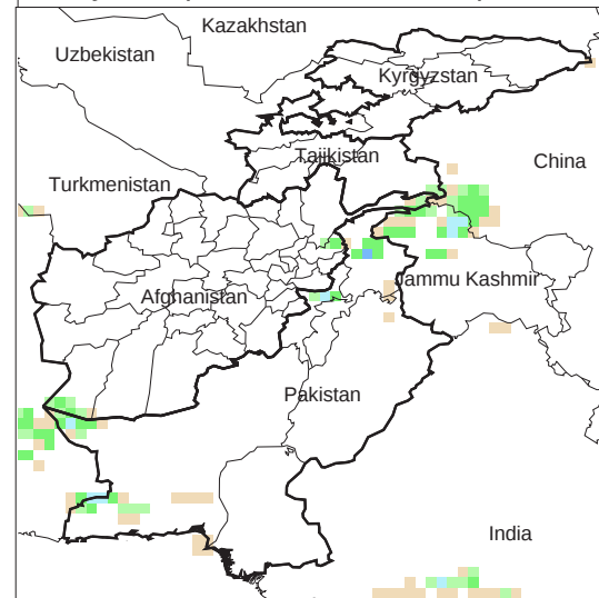
Daily Precip. Forecast for 28 Sep., 2012
