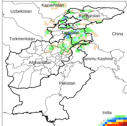
Daily Precip. Forecast for 2 Nov., 2012
