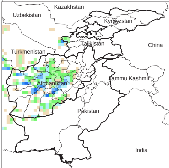
Daily Precip. Forecast for 31 Oct., 2012
