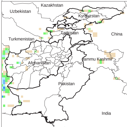
Daily Precip. Forecast for 1 Nov., 2012
