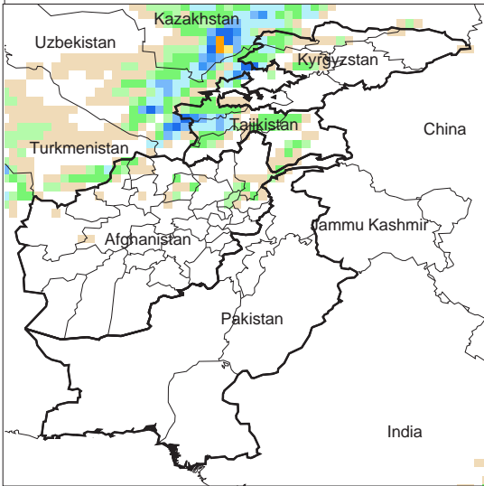
Daily Precip. Forecast for 6 Nov., 2012
