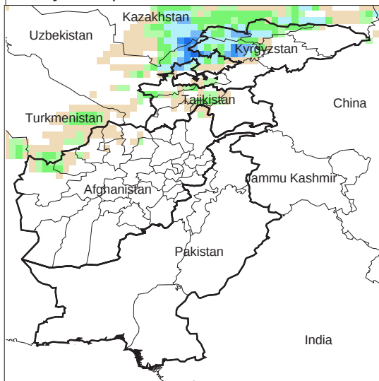
Daily Precip. Forecast for 15 Nov., 2012
