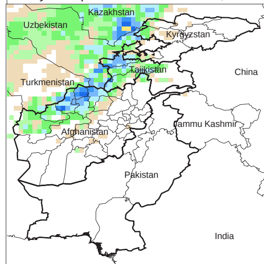
Daily Precip. Forecast for 16 Nov., 2012
