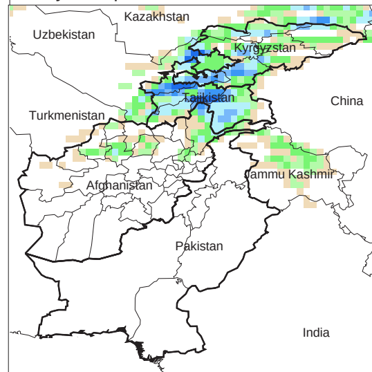
Daily Precip. Forecast for 23 Dec., 2012
