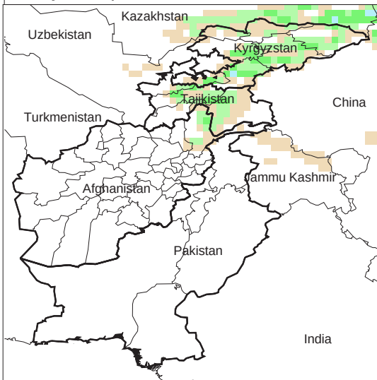
Daily Precip. Forecast for 22 Dec., 2012
