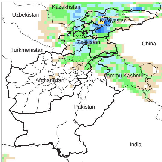
Daily Precip. Forecast for 21 Dec., 2012
