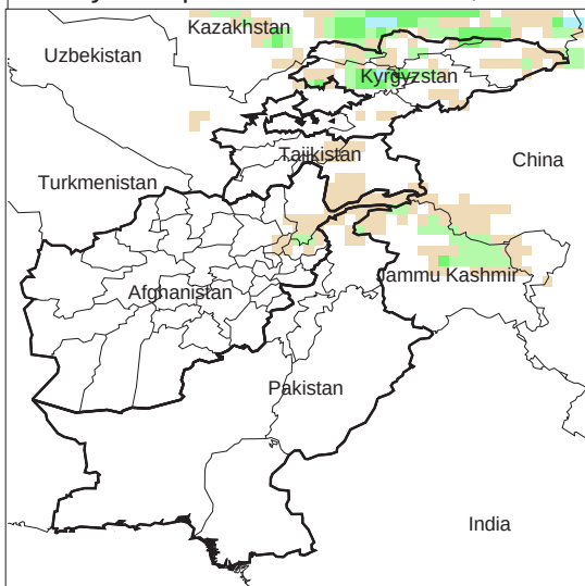
Daily Precip. Forecast for 4 Jan., 2013
