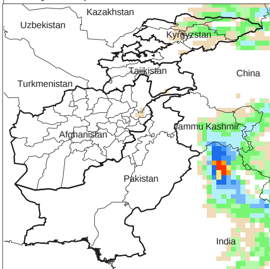
Daily Precip. Forecast for 9 Feb., 2013
