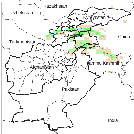
Daily Precip. Forecast for 10 Feb., 2013
