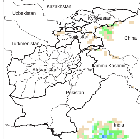
Daily Precip. Forecast for 11 Feb., 2013
